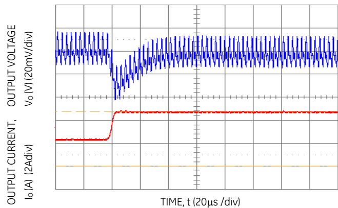
Figure 10. Transient Response to Dynamic Load Change from 50% to 100% at 28Vin, C_{ext} = 10\mu F ceramic + 330 \mu F polymer, C_{Tune}=10nF & R_{Tune}=150\Omega
