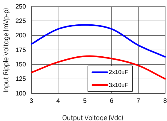
Figure 28. Input ripple voltage for various output voltages with 2x10 μF or 3x10 μF ceramic capacitors at the input (maximum load). Input voltage is 12V.
