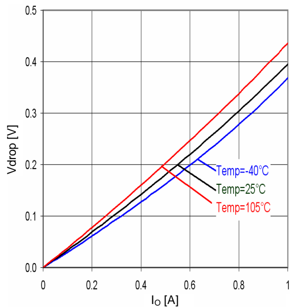
Fig.37 Minimum dropout Voltage 5 (V CC =5.5V, Ta=25°C)
