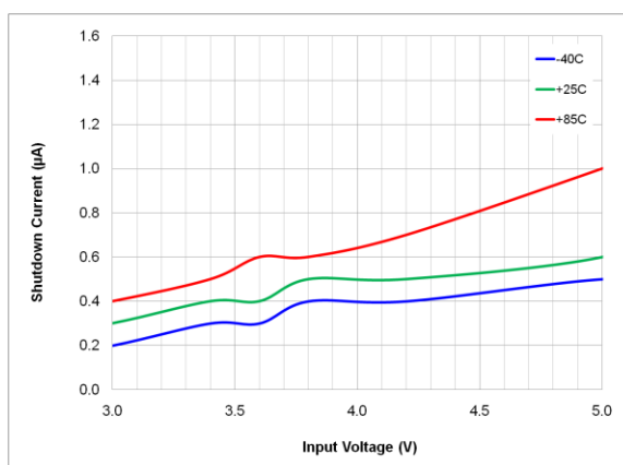
Figure 9. Shutdown Current vs. Input Voltage
