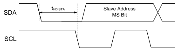
Figure 34. START Bit
