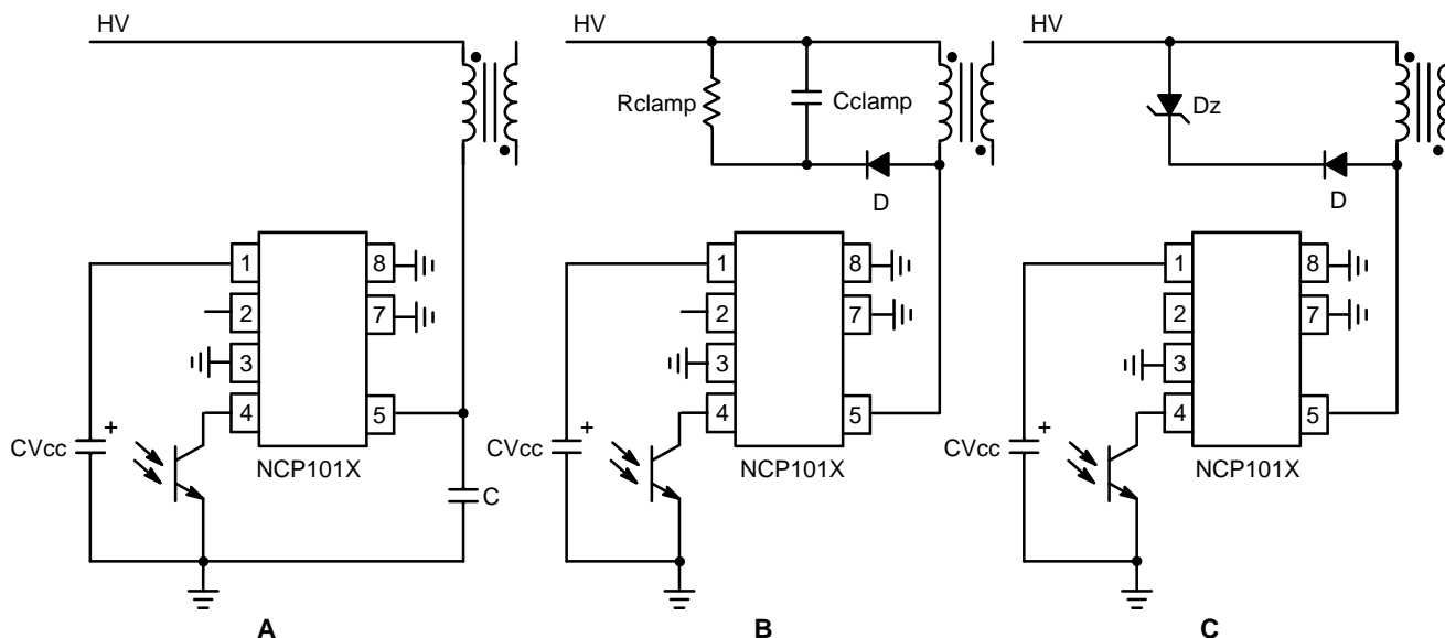
Figure 29. Different Options to Clamp the Leakage Spike
