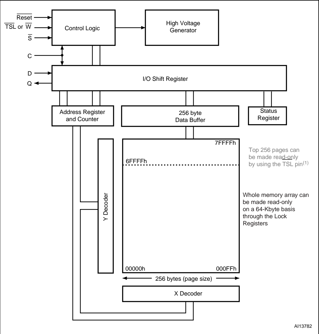
Figure 6. Block diagram
