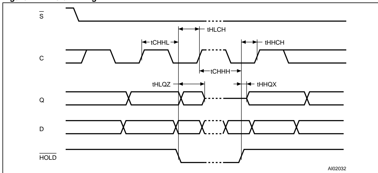
Figure 24. Hold Timing
