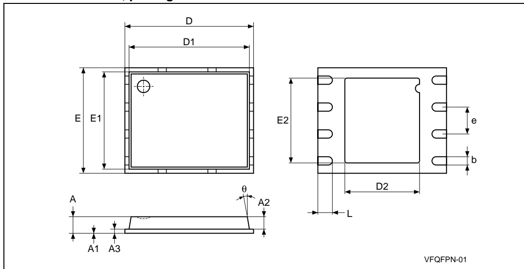
Figure 26. VFQFPN8 (MLP8) 8-lead Very thin Fine Pitch Quad Flat Package No lead, 6x5mm, package outline
