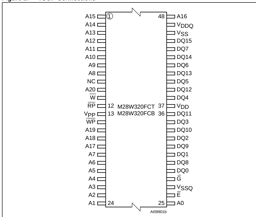
Figure 2. TSOP Connections
