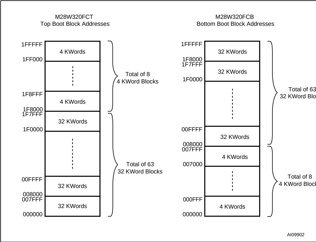
Figure 4. Block Addresses
