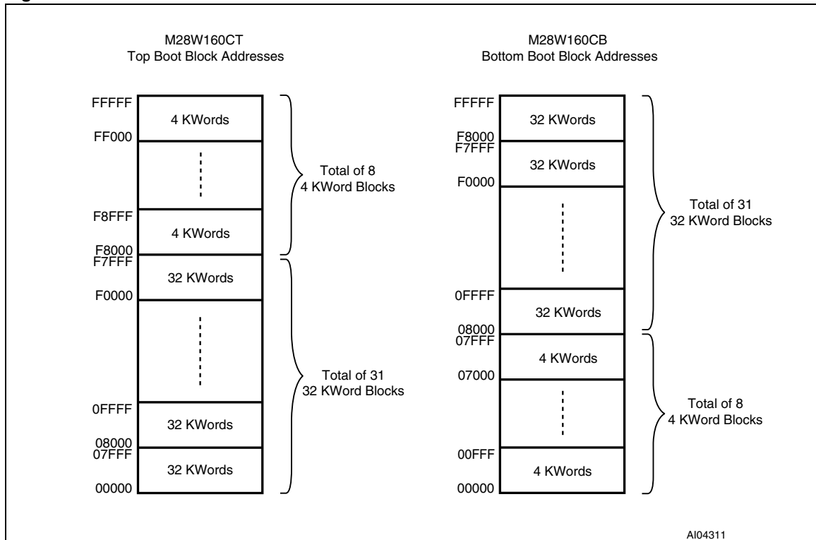
Figure 5. Block Addresses
