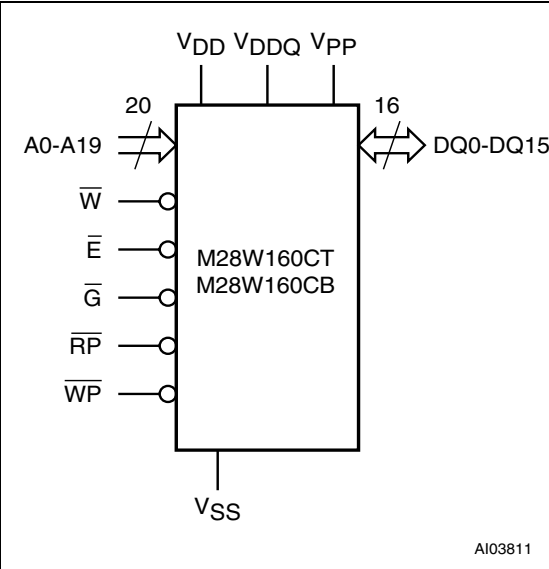
Figure 2. Logic Diagram
