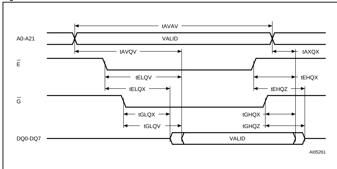
Figure 9. Read AC Waveforms
