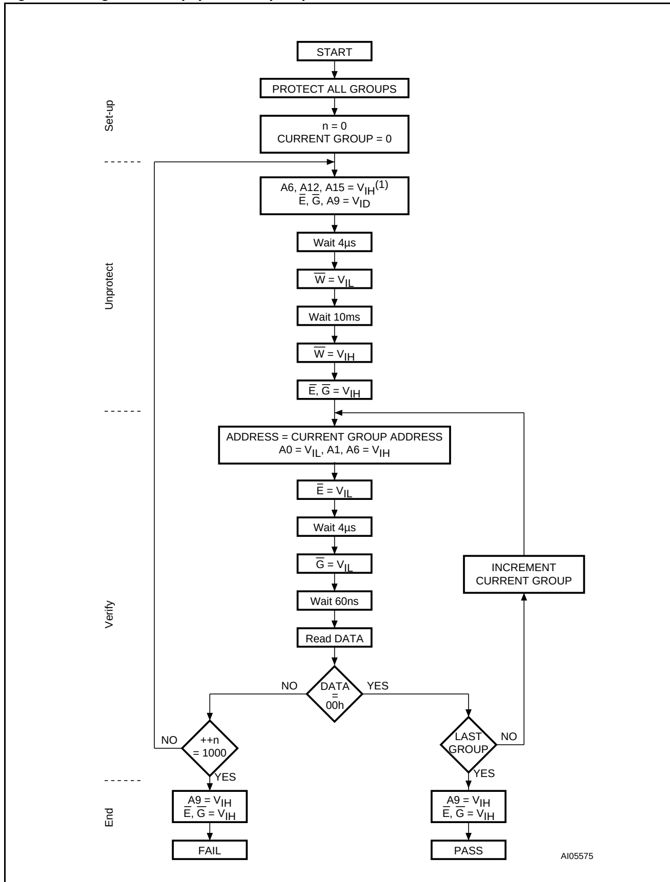
Figure 15. Programmer Equipment Chip Unprotect Flowchart
