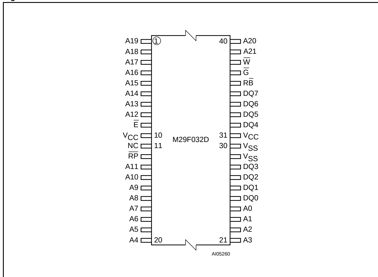
Figure 3. TSOP Connections
