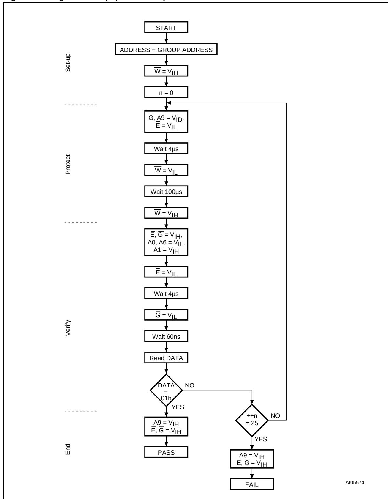
Figure 14. Programmer Equipment Group Protect Flowchart
