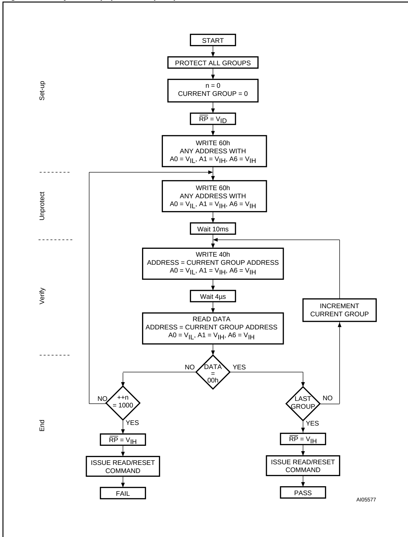
Figure 17. In-System Equipment Chip Unprotect Flowchart
