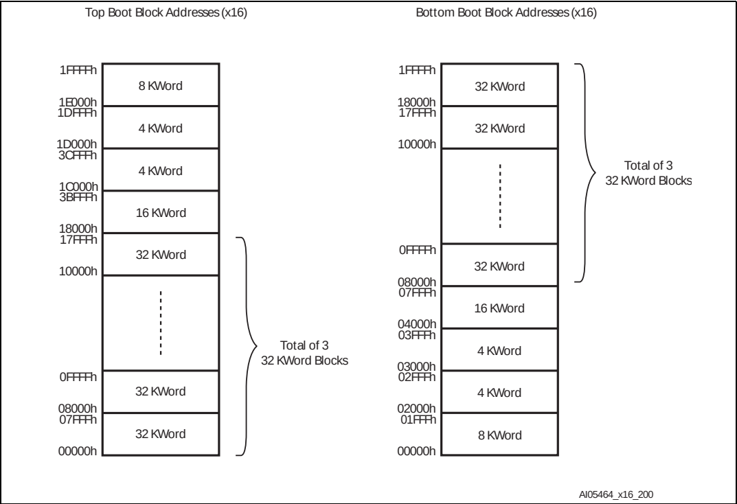
Figure 16. Block Addresses, M29F200 (x16)
