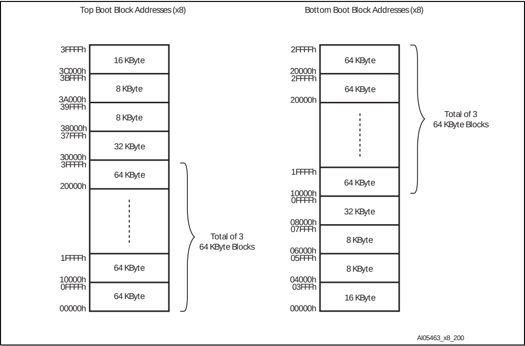
Figure 15. Block Addresses, M29F200 (x8)
