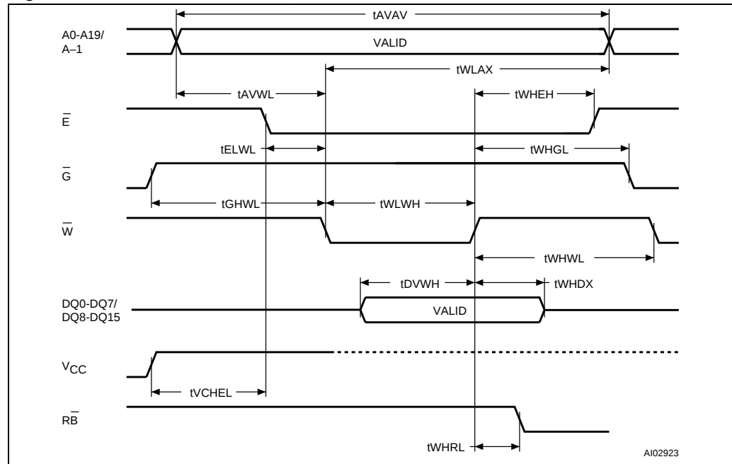
Figure 21. Write AC Waveforms, Write Enable Controlled
