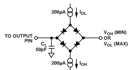
Figure 37. Load Circuit for Measuring V_{OH} and V_{OL} (The diode bridge test circuit is equivalent to the application circuit with R_{PULL-UP} of 2.2 kΩ.)
