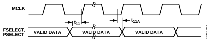
Figure 4. Control Timing
