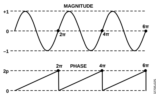
Figure 27. Sine Wave
