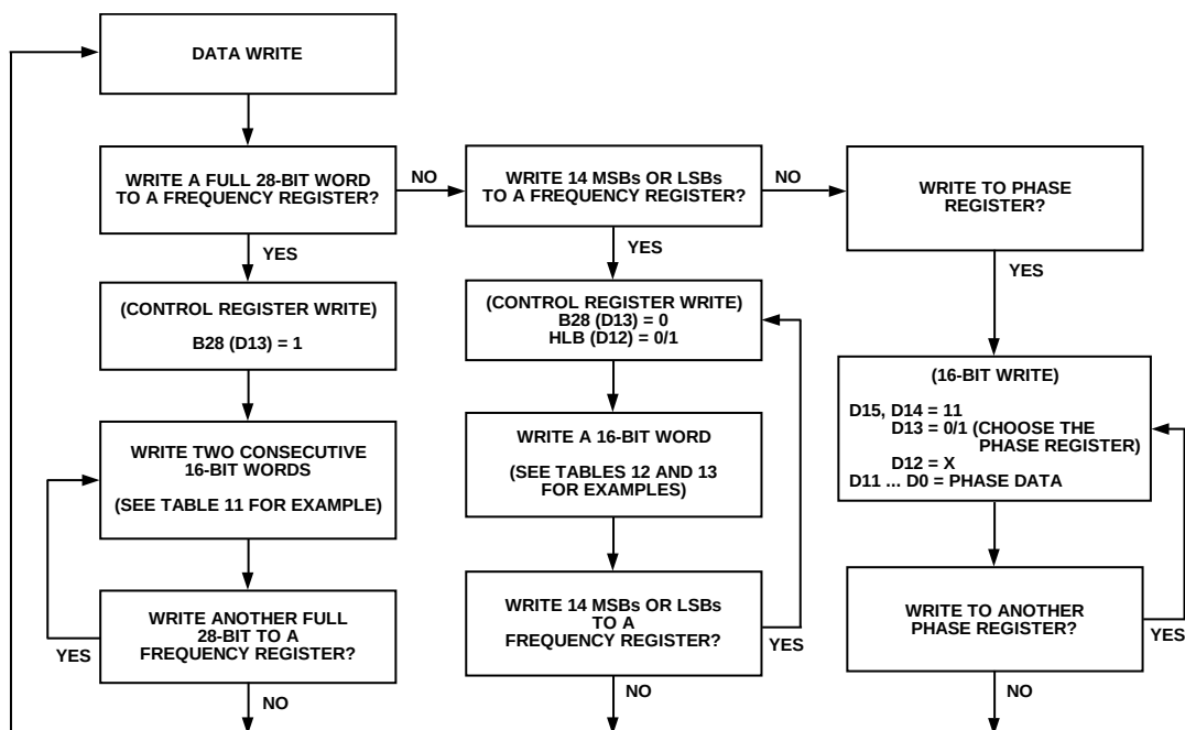
Figure 33. Data Write
