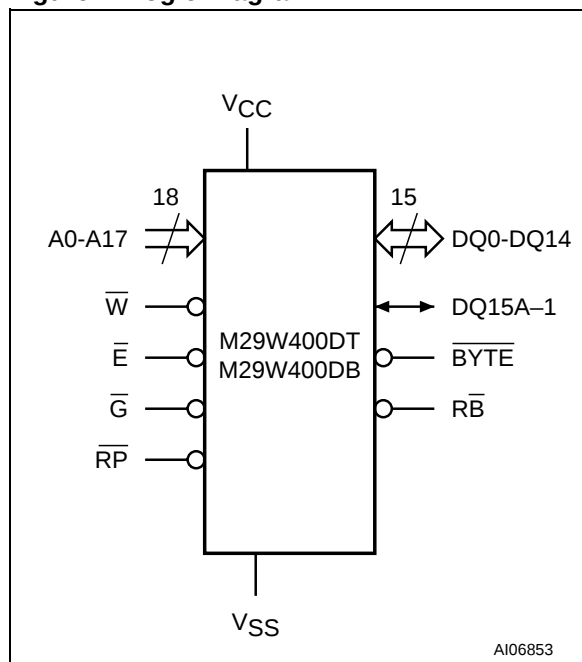
Figure 2. Logic Diagram
