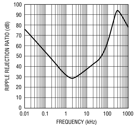
2.5V Ripple Rejection Ratio vs Frequency
