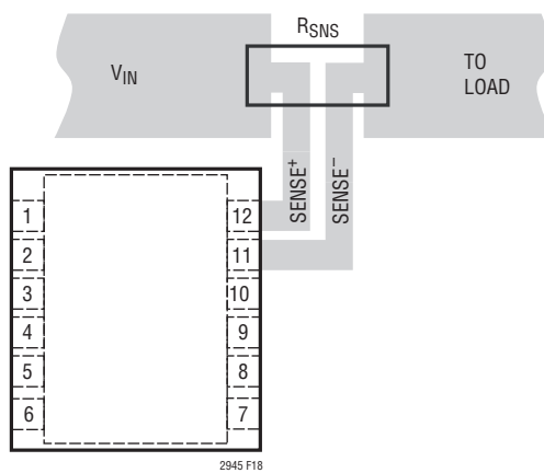
Figure 18. Recommended Layout for Kelvin Connection
