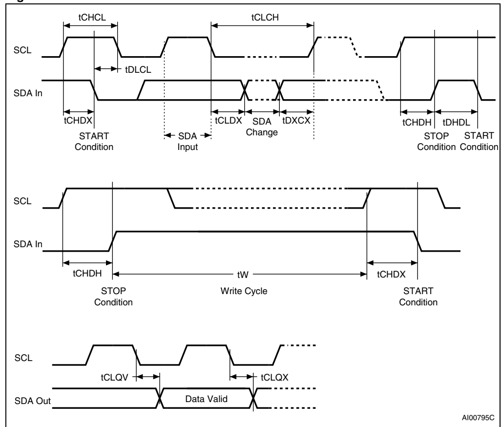
Figure 13. AC waveforms
