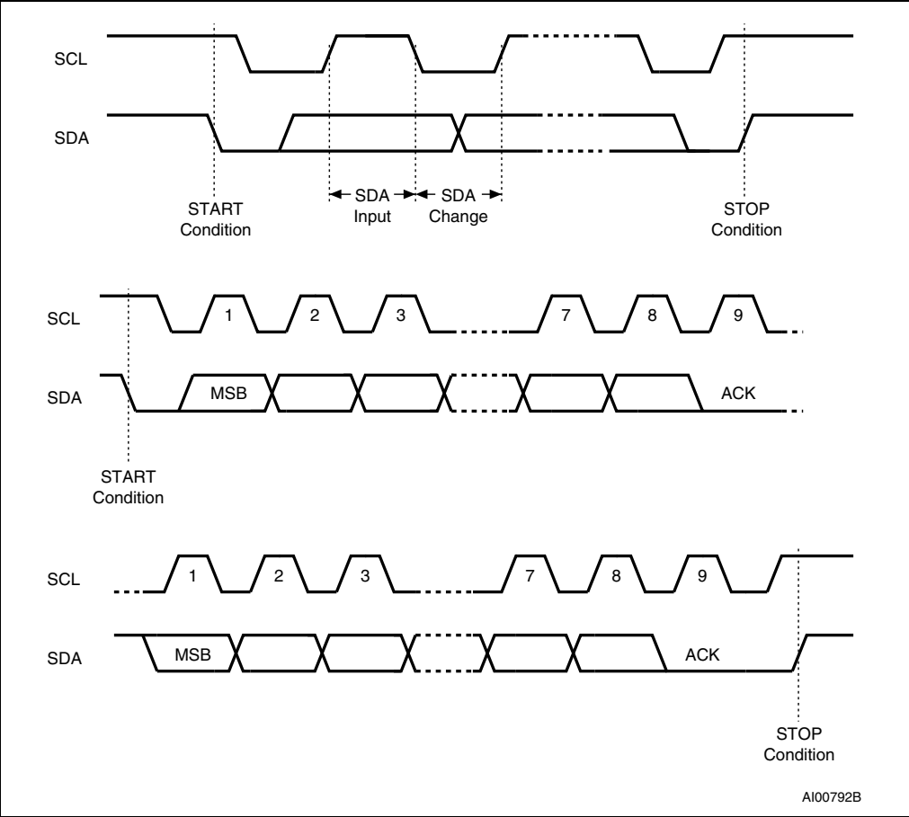
Figure 5. I 2 C bus protocol
