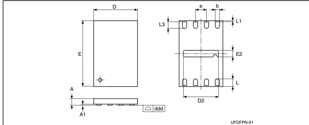
Figure 14. UDFFPN8 (MLP8) 8-lead ultra thin fine pitch dual flat package no lead 2 x 3 mm, package outline
