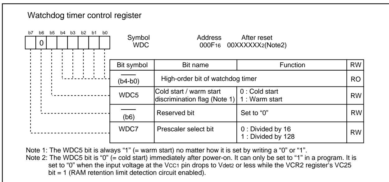
Figure 1.5.5. WDC Register
