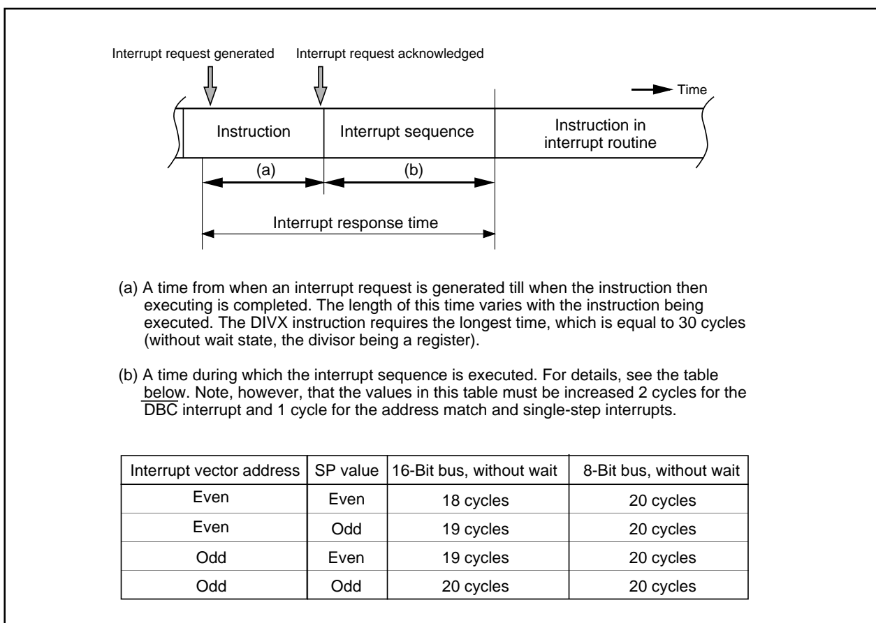
Figure 1.11.5. Interrupt response time
