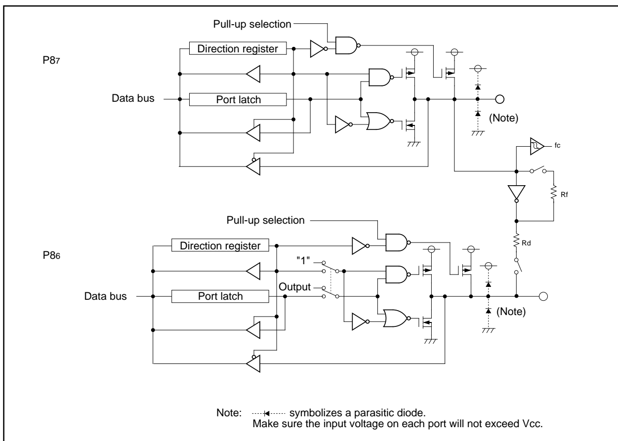
Figure 1.25.5. I/O Ports (5)
