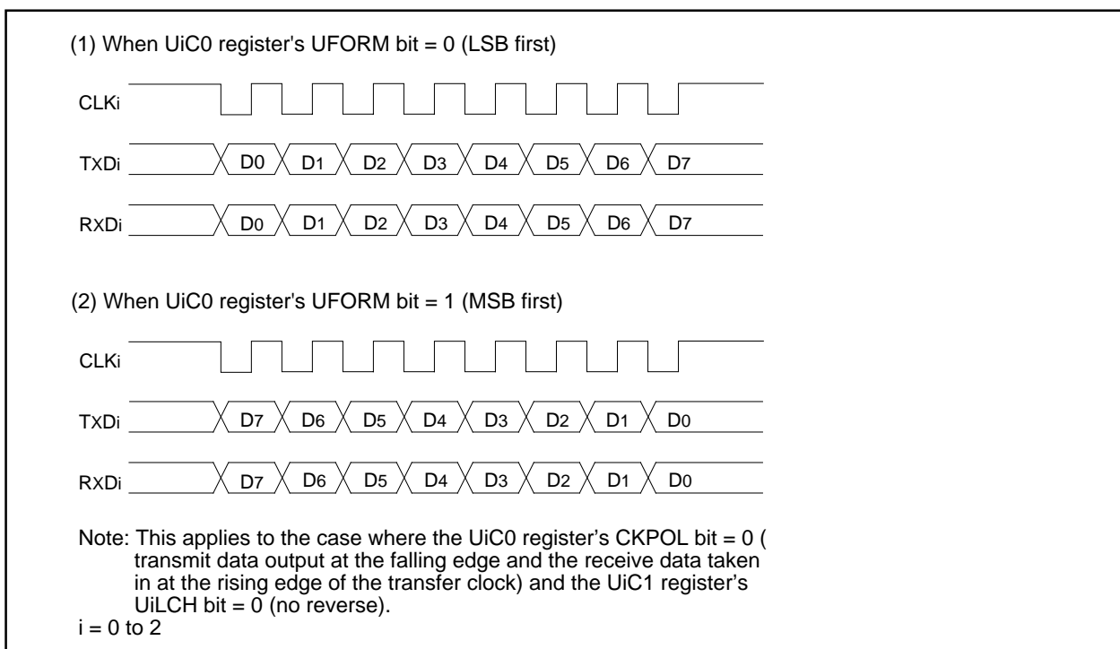
Figure 1.18.3. Transfer Format
