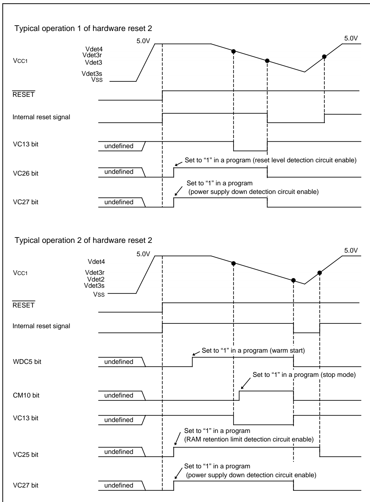
Figure 1.5.7. Typical Operation of Hardware Reset 2
