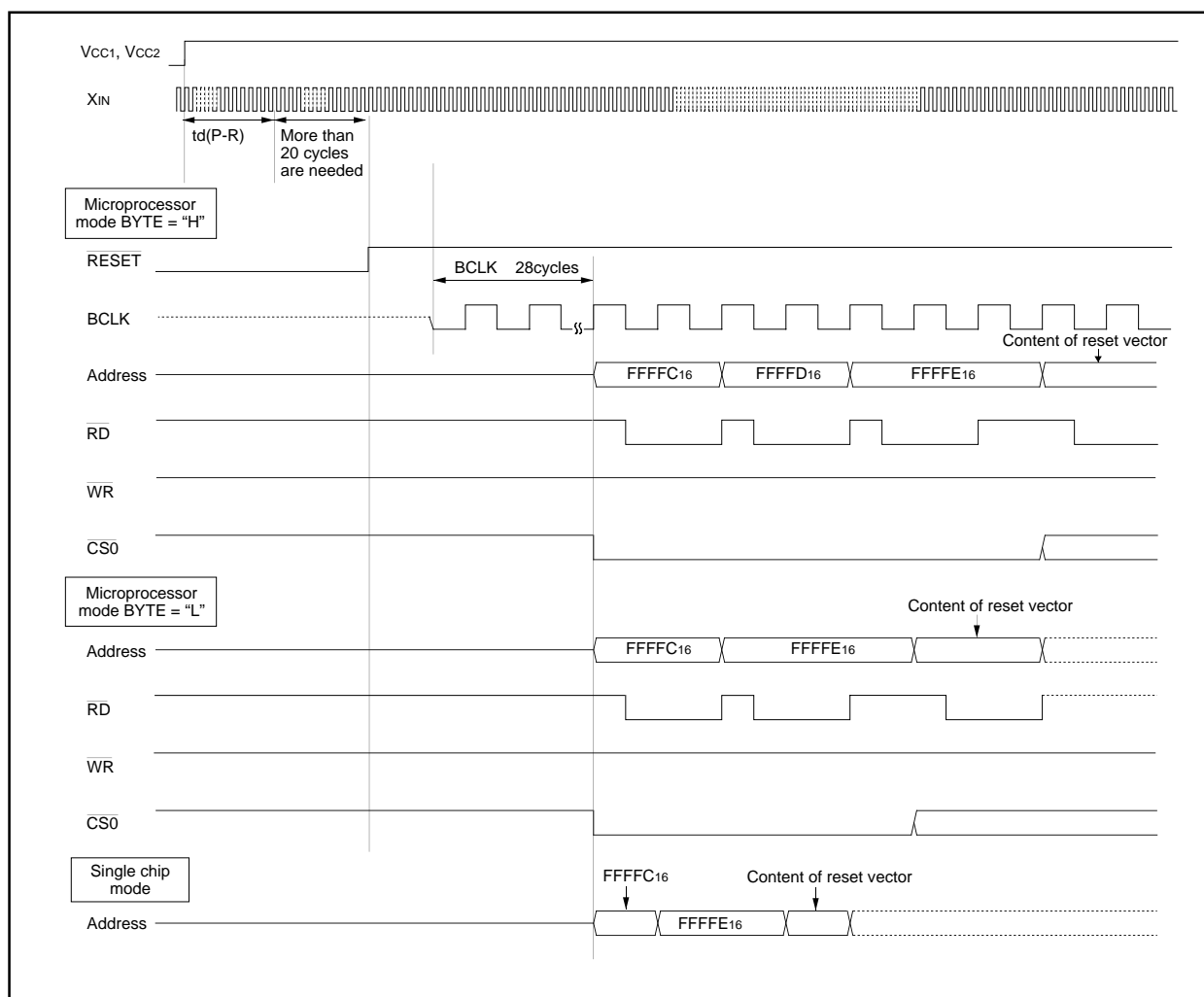
Figure 1.5.2. Reset Sequence
