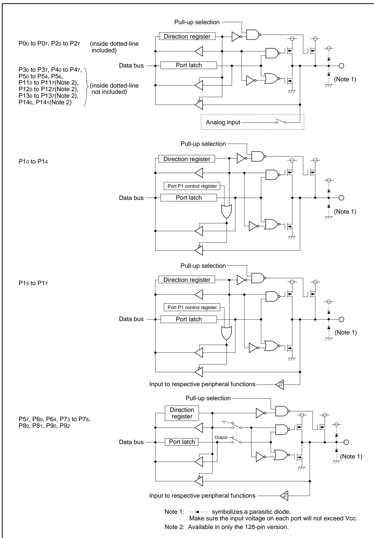
Figure 1.25.1. I/O Ports (1)
