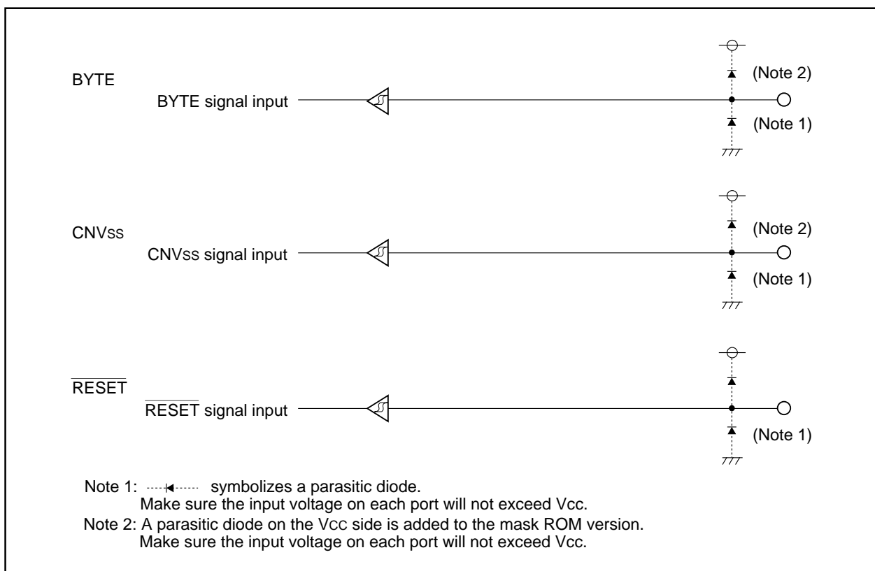
Figure 1.25.6. I/O Pins
