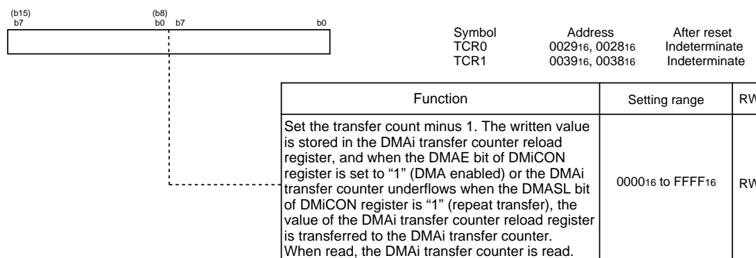
Figure 1.13.4. SAR0, SAR1, DAR0, DAR1, TCR0, and TCR1 Registers
