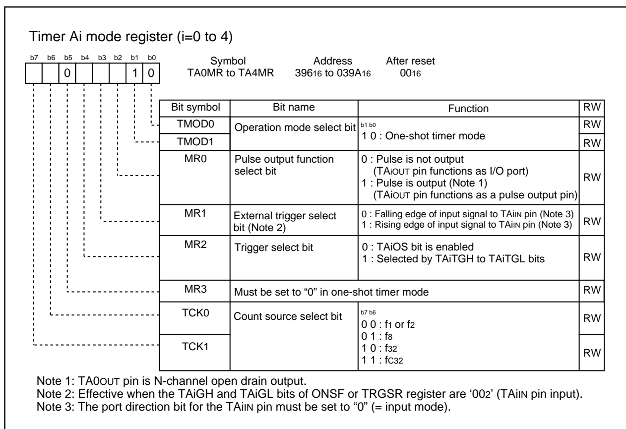
Figure 1.14.12. TAIiMR Register in One-shot Timer Mode
