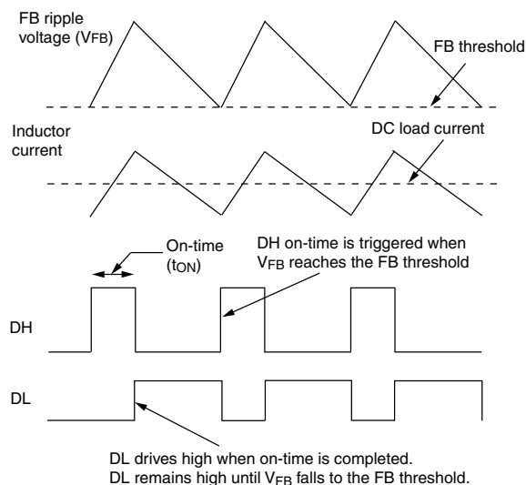
Fig. 26 - Forced Continuous Mode Operation
