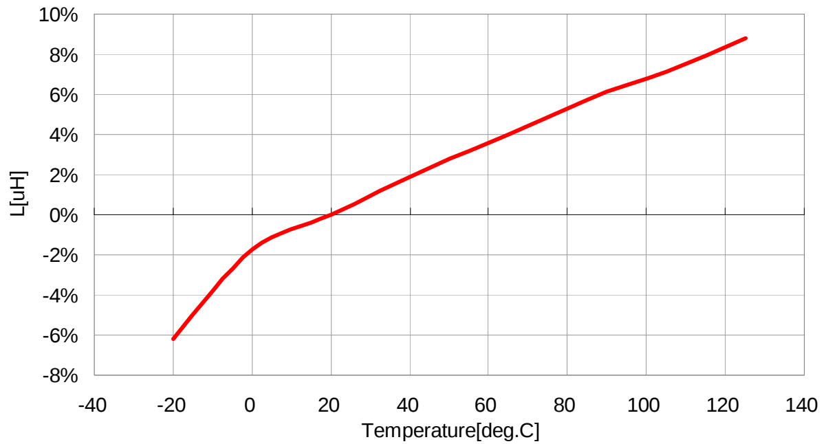
VLS3012T-220MR49
