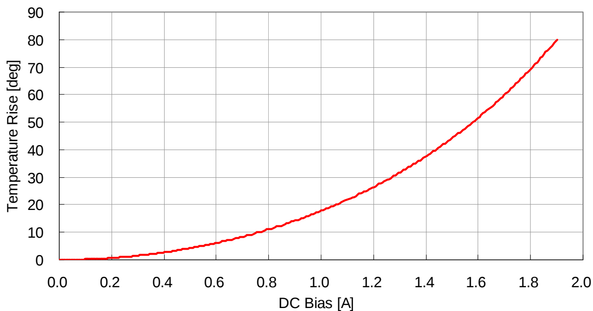
VLS3012T-6R8MR90
