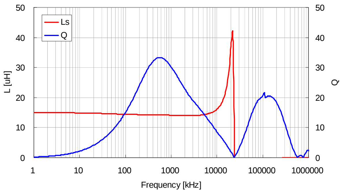
VLS3012T-150MR58
