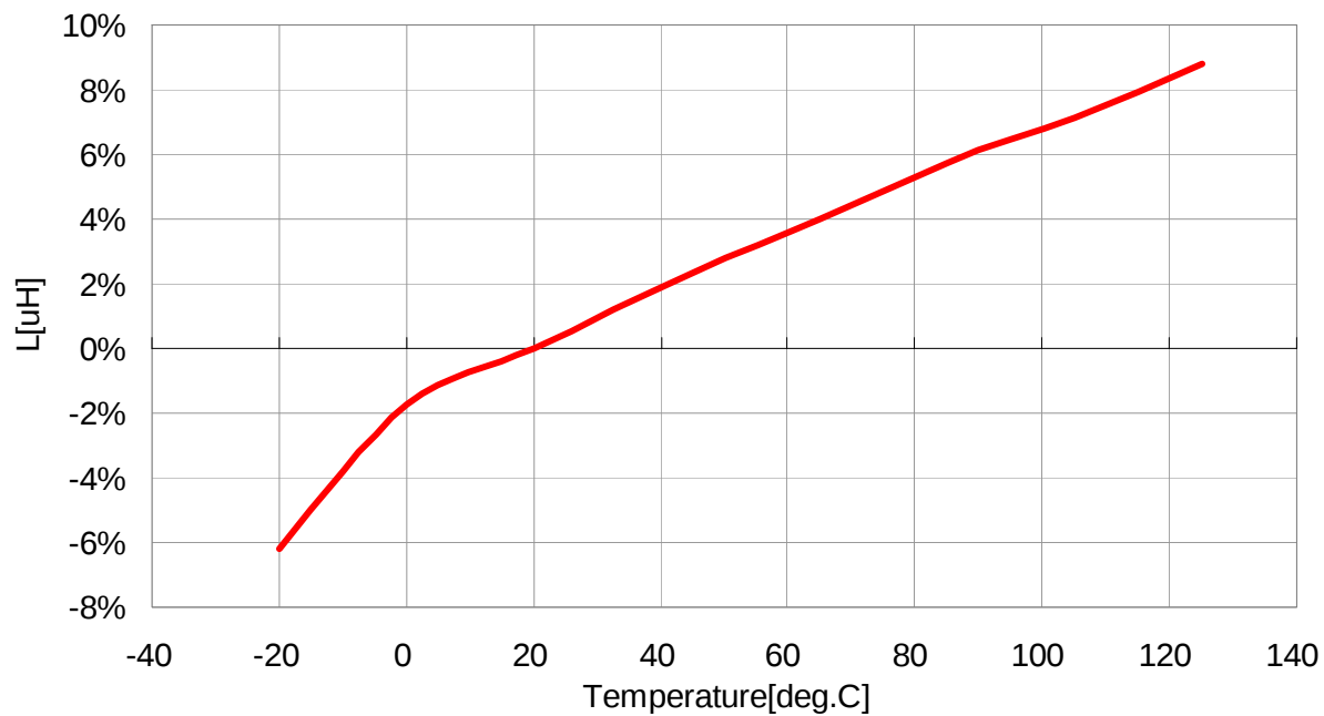
VLS3012T-100MR72
