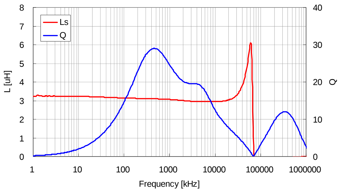
VLS3012T-3R3M1R3
