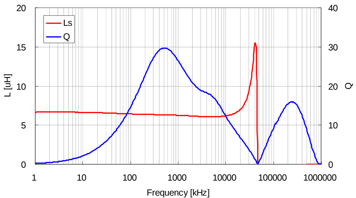
VLS3012T-6R8MR90
