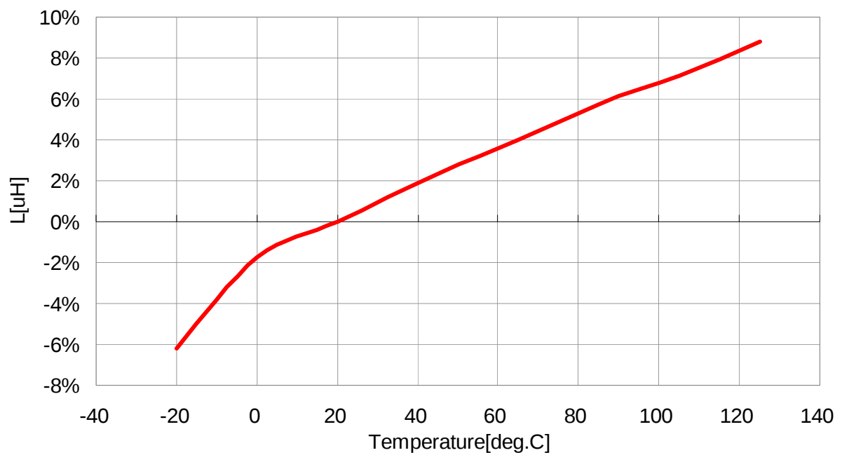
VLS3012T-6R8MR90
