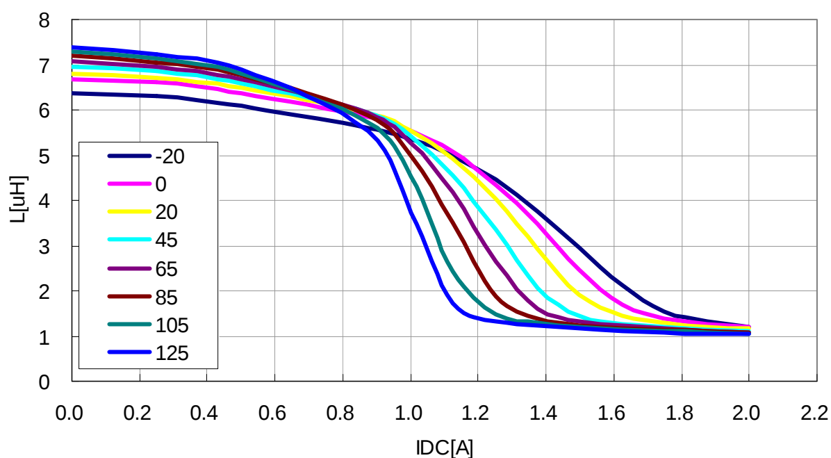
VLS3012T-6R8MR90
