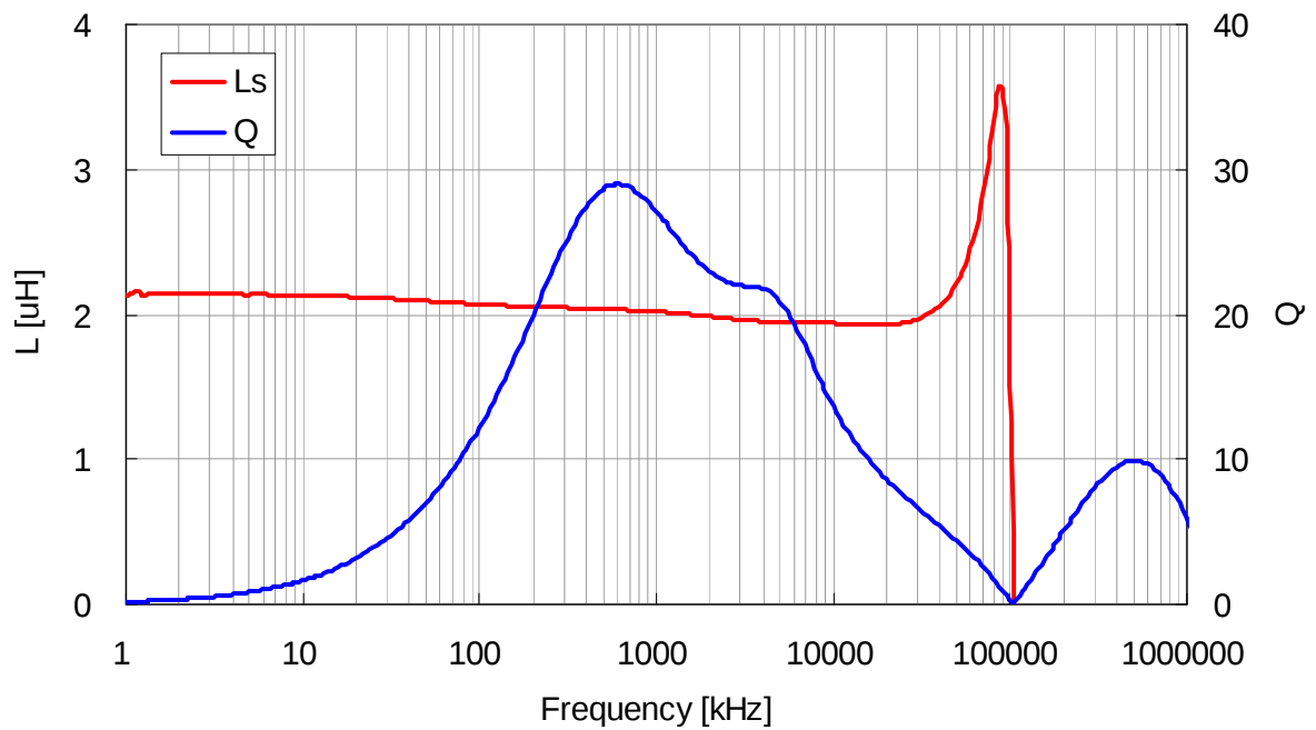
VLS3012T-2R2M1R5
