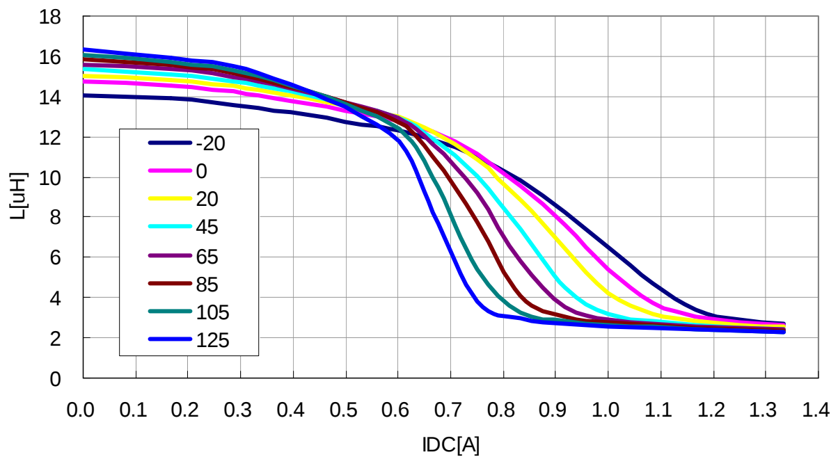
VLS3012T-150MR58
