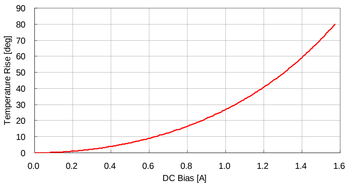
VLS3012T-6R8MR90
