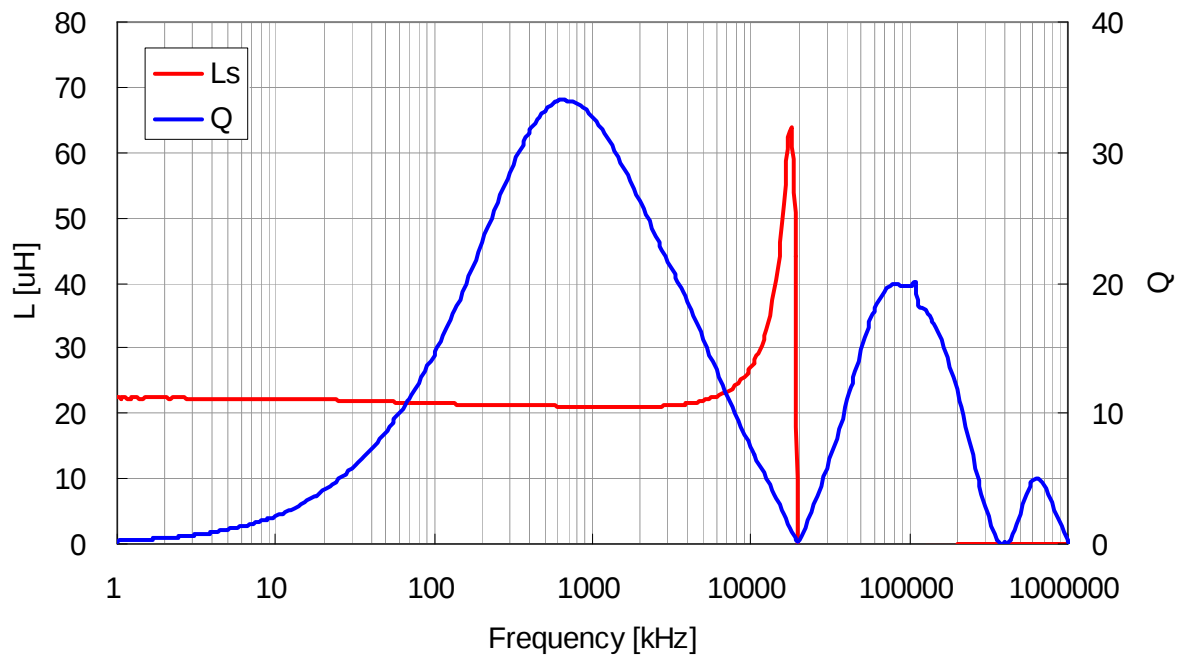
VLS3012T-220MR49
