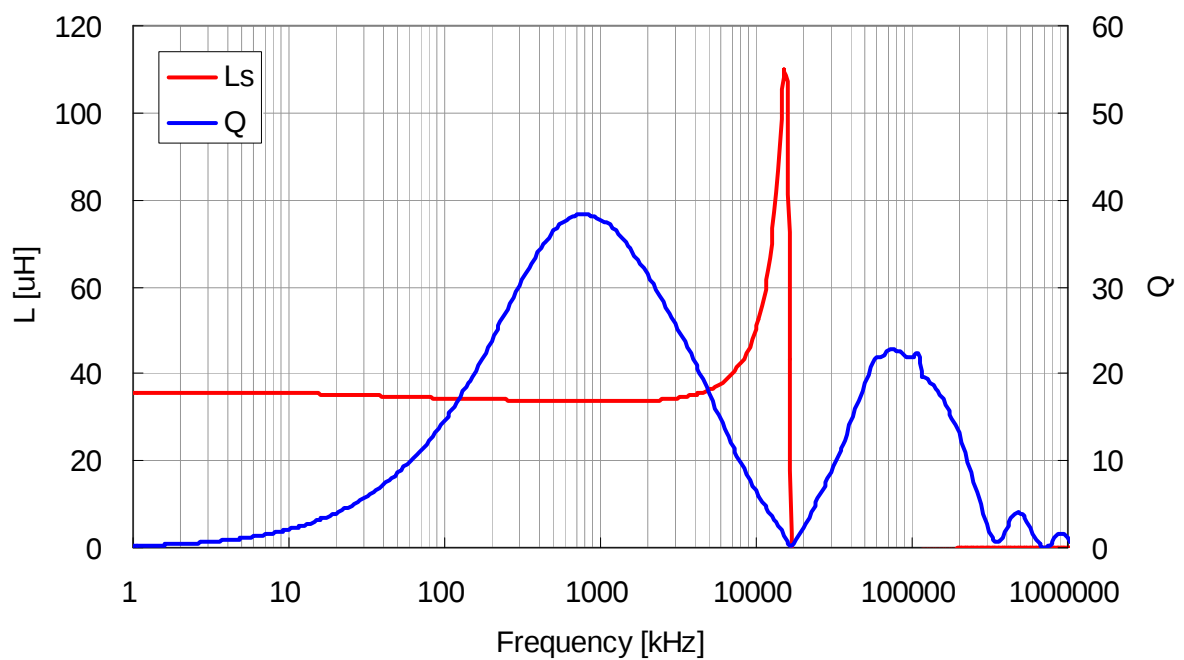
VLS3012T-330MR40
