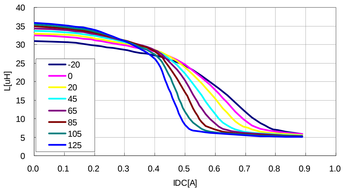
VLS3012T-330MR40
