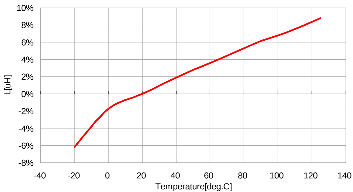
VLS3012T-150MR58
