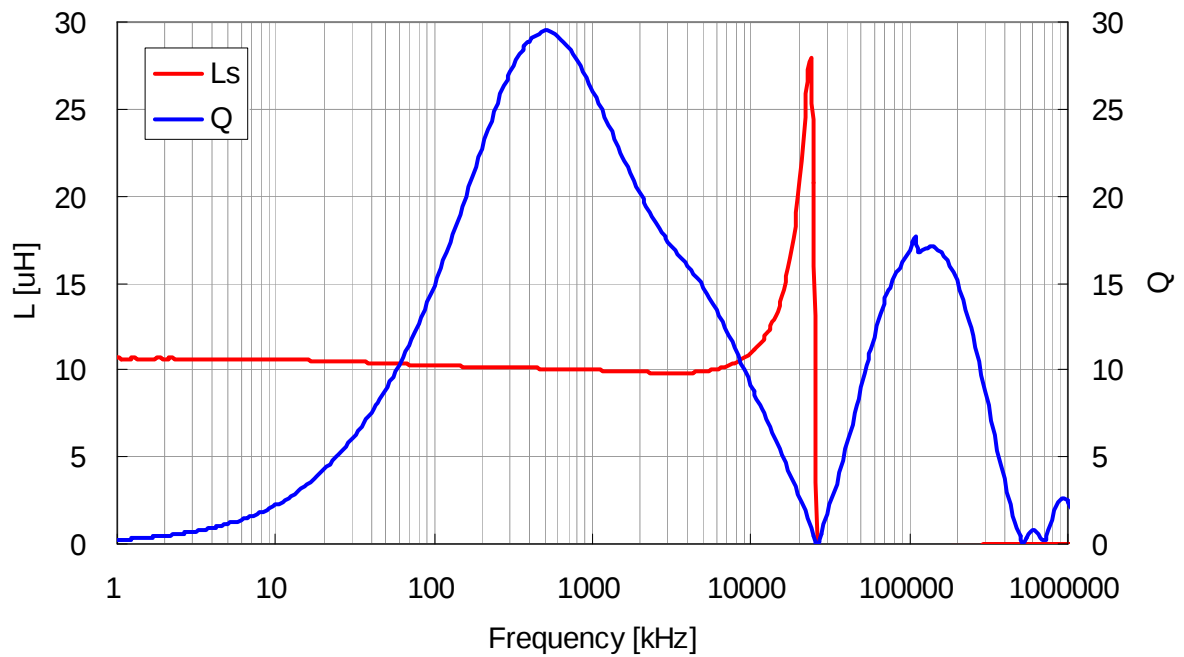
VLS3012T-100MR72
