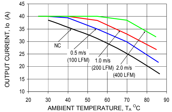
Figure 34. Derating Output Current versus Local Ambient Temperature and Airflow (direction shown in Figure 63).
