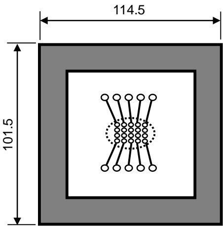
Standard Test Land Pattern
