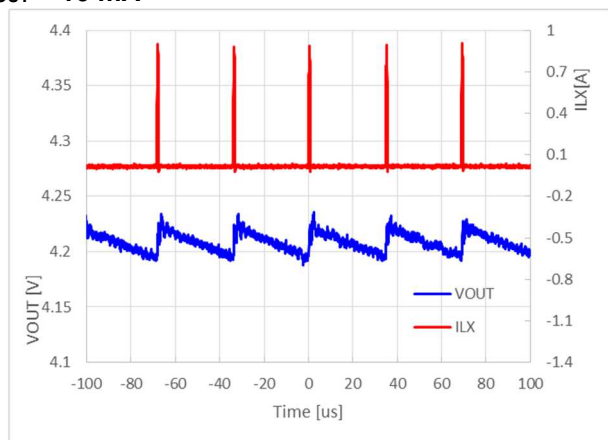
RP602Z420x, V_{IN} = 3.6\text{ V} , MODE = H I_{OUT} = 10\text{ mA}
