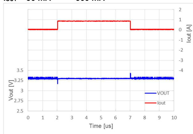
RP602Z330x, V_{IN} = 3.6\text{ V} , MODE = L I_{OUT} = 50\text{ mA} \leftrightarrow 900\text{ mA}
