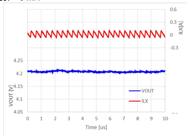
RP602Z420x, V_{IN} = 3.6\text{ V} , MODE = L I_{OUT} = 0\text{ mA}
