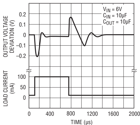
LT1761-5 Transient Response C_{BYP} = 0pF
