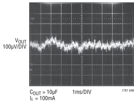
LT1761-5 10Hz to 100kHz Output Noise C_{BYP} = 1000pF
