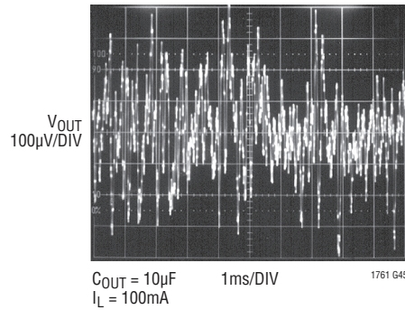
LT1761-5 10Hz to 100kHz Output Noise C_{BYP} = 0pF
