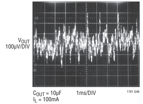
LT1761-5 10Hz to 100kHz Output Noise C_{BYP} = 100pF
