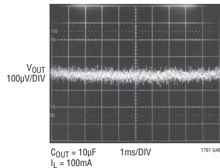
LT1761-5 10Hz to 100kHz Output Noise C_{BYP} = 0.01µF
