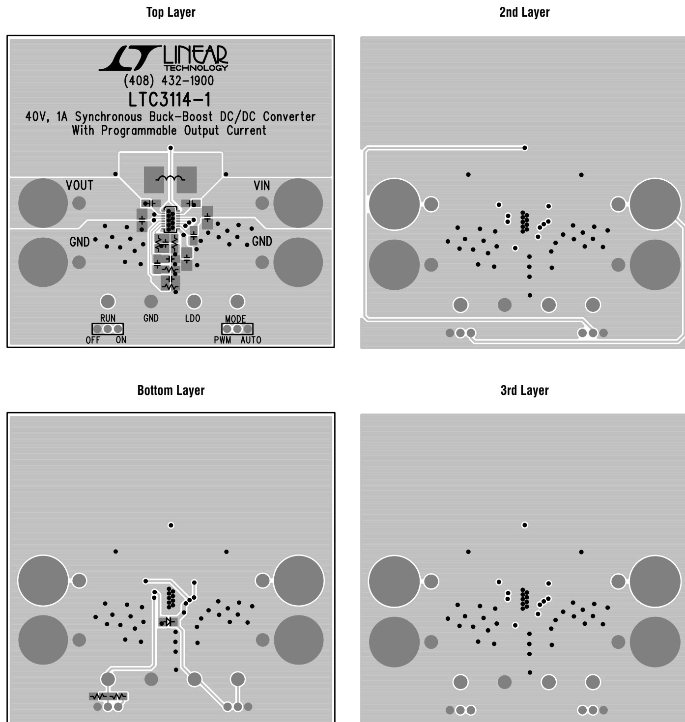
Figure 4. Typical 4 Layer PC Board Layout
