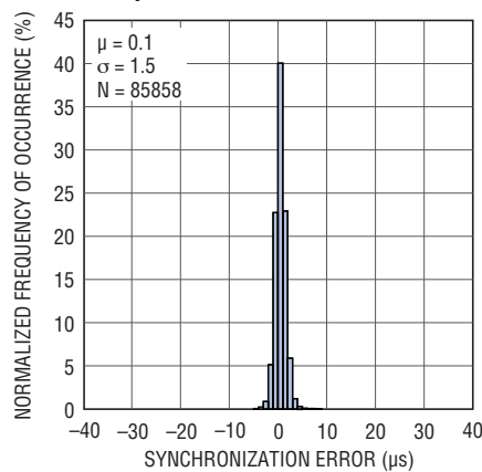
TIME n Synchronization Error 1 Packet/s Publishing Rate, 3 Hops, 2°C/Min
