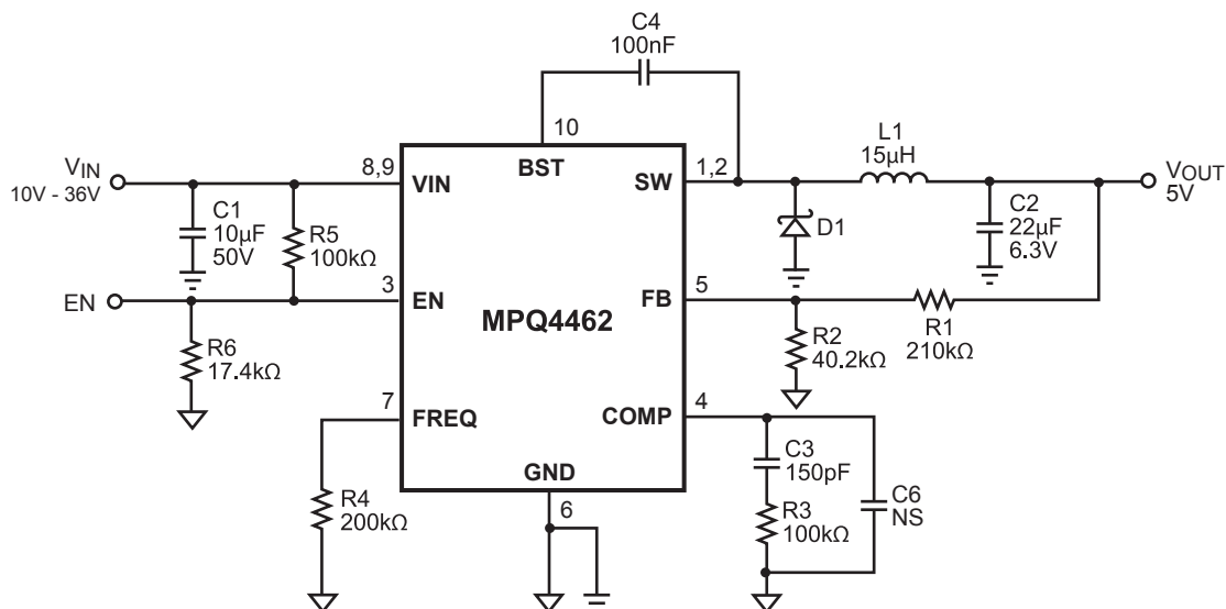
Figure 5: Typical Application, 5V Output
