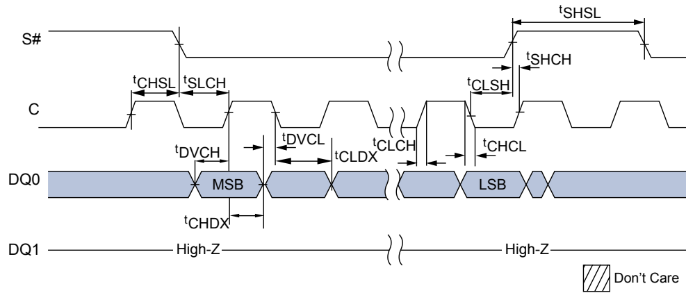
Figure 44: Serial Input Timing DTR
