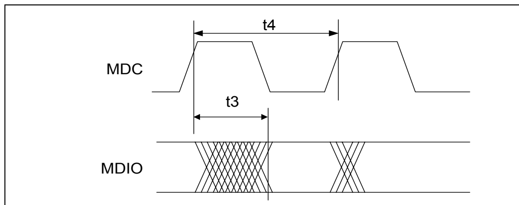
Figure 30 MDIO Output Timing
