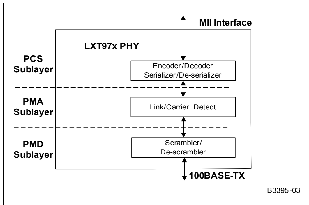
Figure 17 Protocol Sublayers
