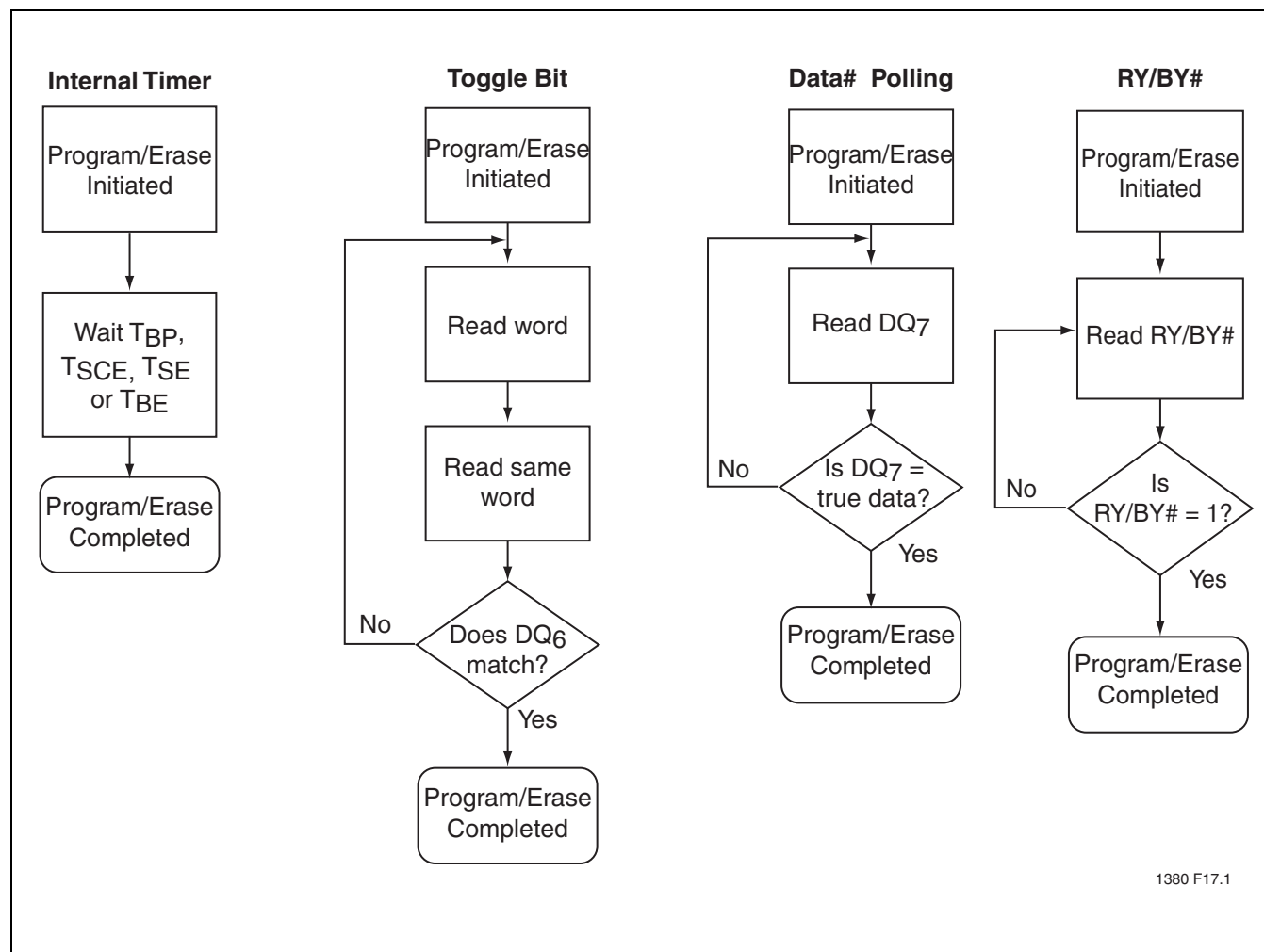
FIGURE 22: Wait Options
