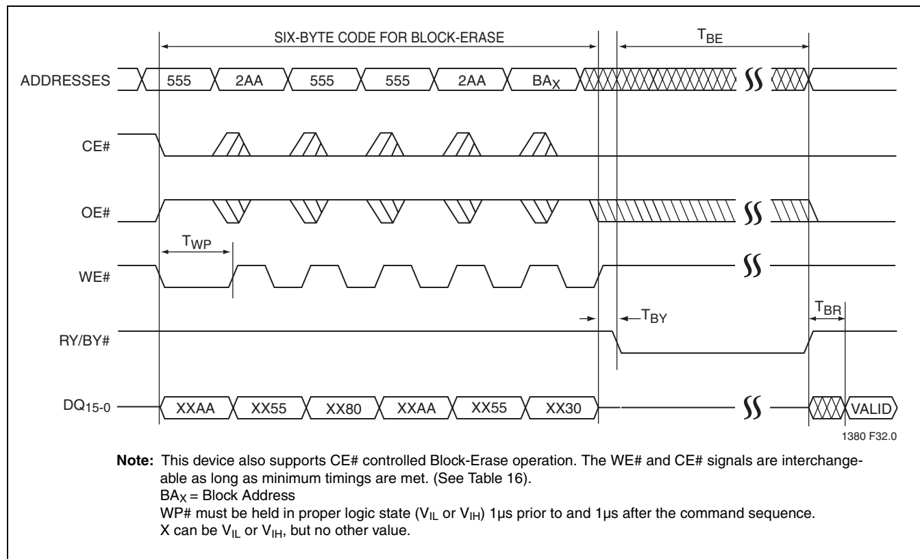
FIGURE 11: WE# Controlled Block-Erase Timing Diagram
