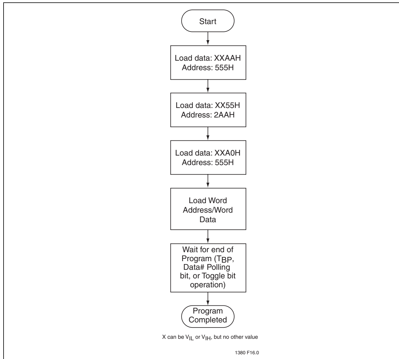
FIGURE 21: Word-Program Algorithm
