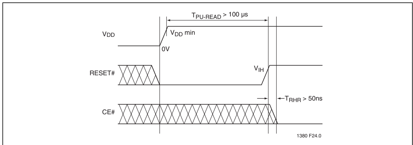
FIGURE 4: Power-Up Diagram
