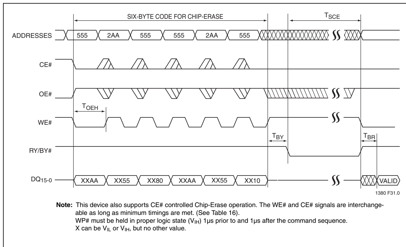
FIGURE 10: WE# Controlled Chip-Erase Timing Diagram
