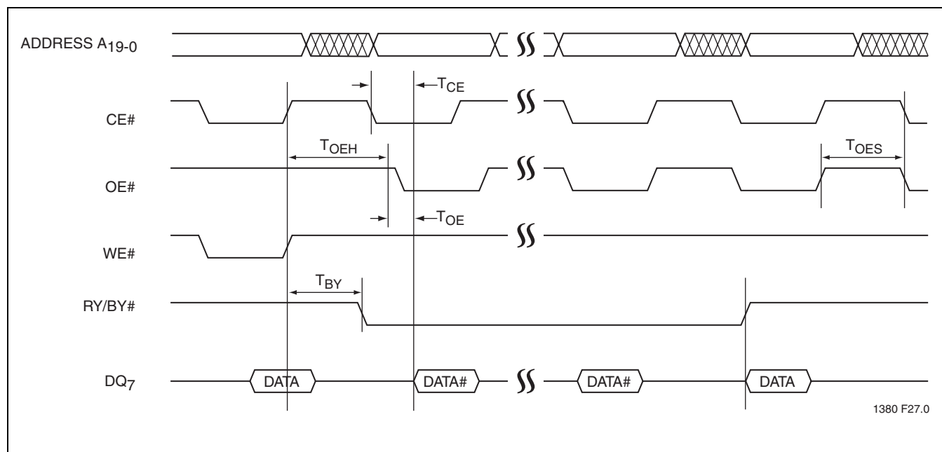
FIGURE 8: Data# Polling Timing Diagram
