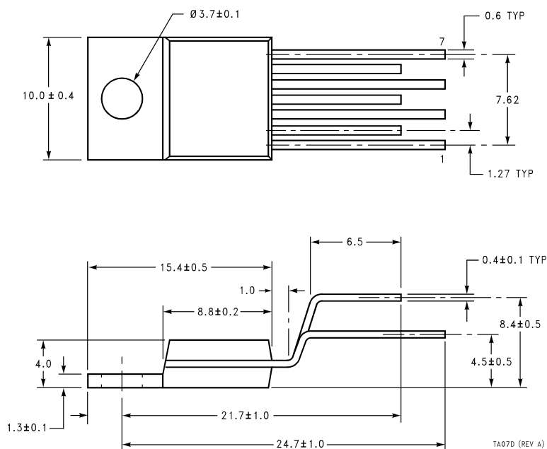
7-Lead Molded TO-220 Order Number LM9070T/Flow LB09 NS Package Number TA07D
