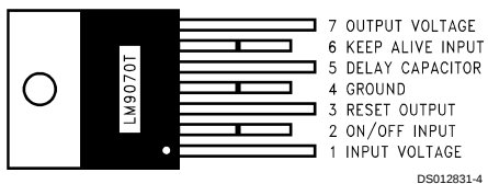
7-Lead TO-220 Package (Even numbered pins bent forward away from package body)
