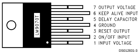
7-Lead TO-220 Package (Odd numbered pins bent forward away from package body)
