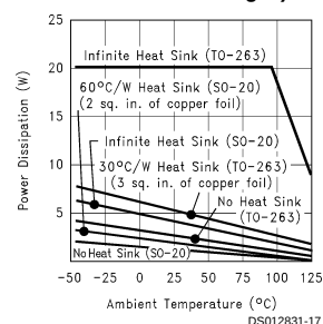
Maximum Power Dissipation (TO-263 and SO-20 Packages)
