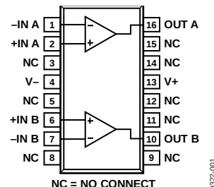
Figure 1. 16-Lead SOIC (S-Suffix)
