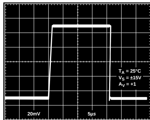
Figure 28. Small Signal Transient Response
