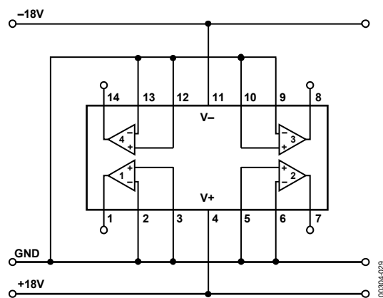
Figure 30. Burn-In Circuit
