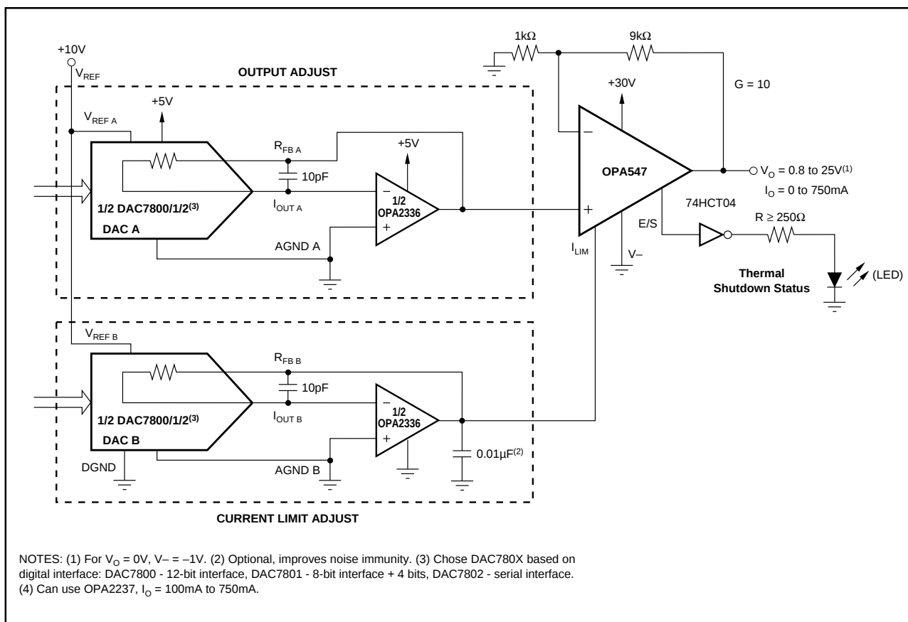
FIGURE 14. Digitally-Controlled Programmable Power Supply.
