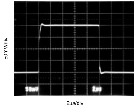
SMALL SIGNAL STEP RESPONSE G = 1 , C_L = 1000\text{pF}
