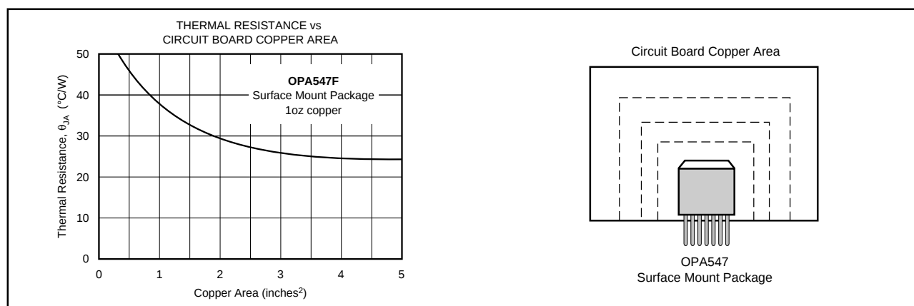
FIGURE 4. Thermal Resistance vs. Circuit Board Copper Area.
