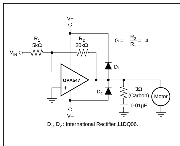
FIGURE 11. Motor Drive Circuit.
