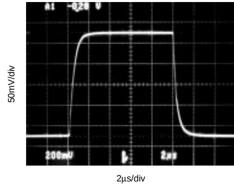
SMALL SIGNAL STEP RESPONSE G = 3 , C_L = 1000\text{pF}
