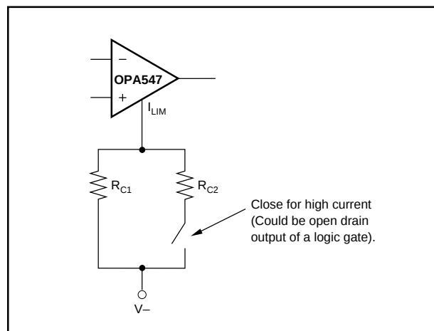
FIGURE 16. Multiple Current Limit Values.
