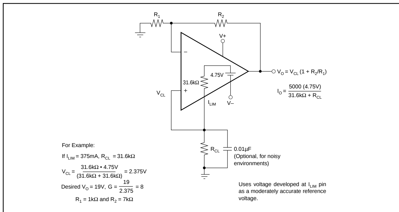
FIGURE 12. Voltage Source.
