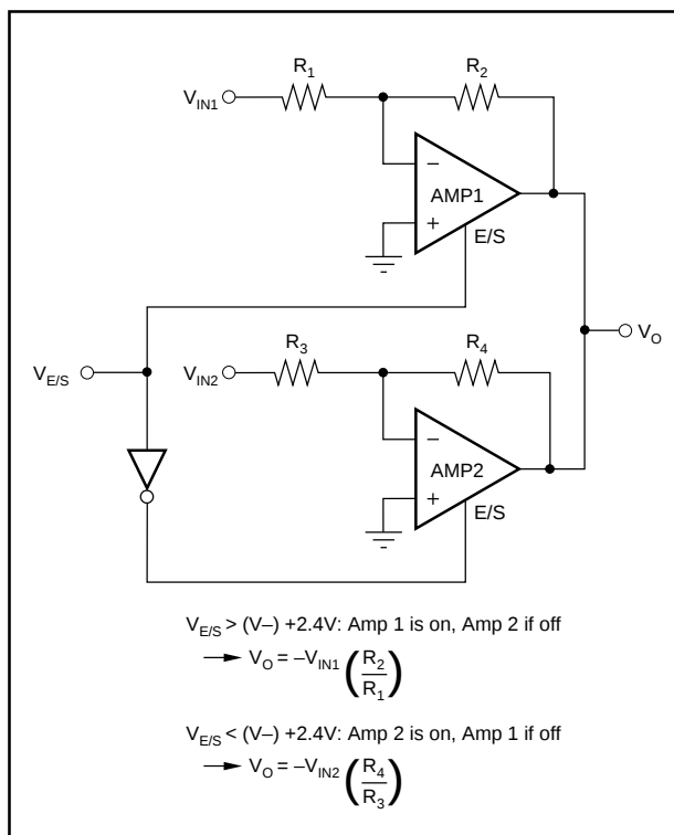
FIGURE 15. Swap Amplifier.
