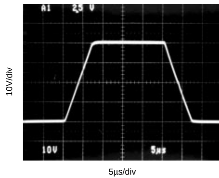
LARGE SIGNAL STEP RESPONSE G = 3 , C_L = 100\text{pF} , R_L = 50\Omega
