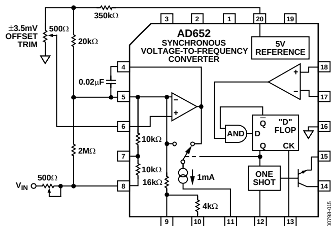
Figure 15. PLCC Gain and Offset Trim
