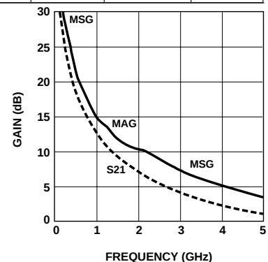
Figure 17. AT-41533 Gains vs. Frequency at V_{CE} = 5\text{ V} , I_C = 25\text{ mA} .
