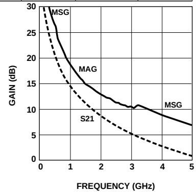
Figure 16. AT-41511 Gains vs. Frequency at V_{CE} = 5\text{ V} , I_C = 25\text{ mA} .
