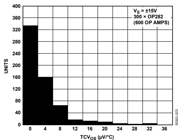
Figure 24. OP282 TCOS Distribution, SOIC_N Package
