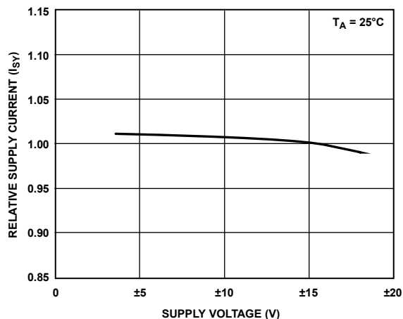
Figure 34. OP482 Relative Supply Current vs. Supply Voltage
