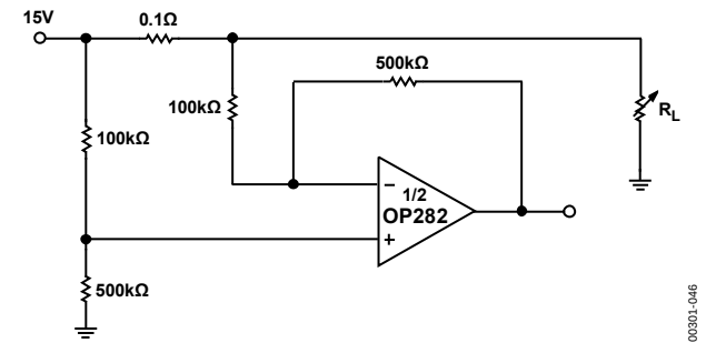
Figure 45. High-Side Signal Conditioning
