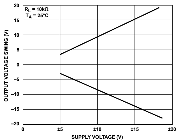
Figure 35. OP482 Output Voltage Swing vs. Supply Voltage
