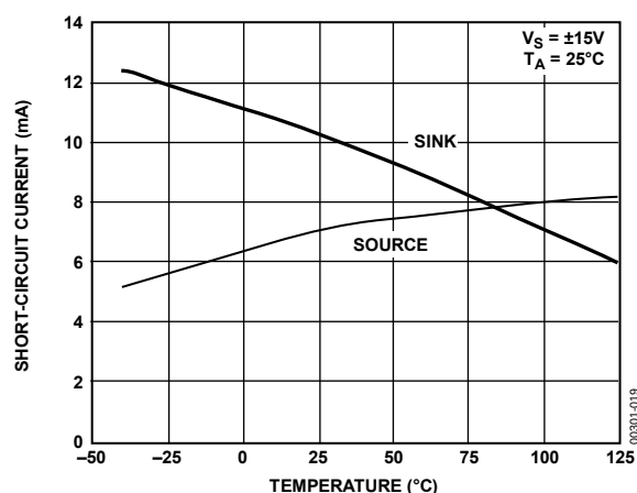
Figure 20. OP282 Short-Circuit Current vs. Temperature
