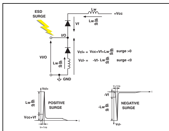
Figure 4. Surge behavior
