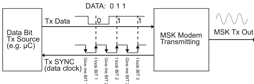
Figure 4 Synchronous Transmit Operation
