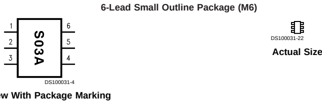
Top View With Package Marking
