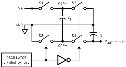
FIGURE 2. Voltage Inverting Principle
