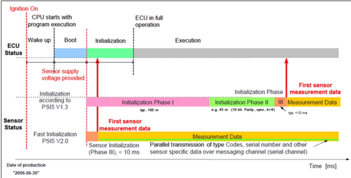
Figure 19. Timing diagram
