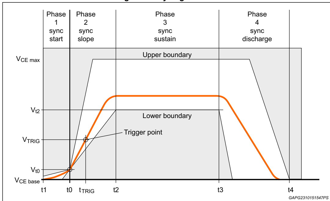
Figure 30. Sync generator
