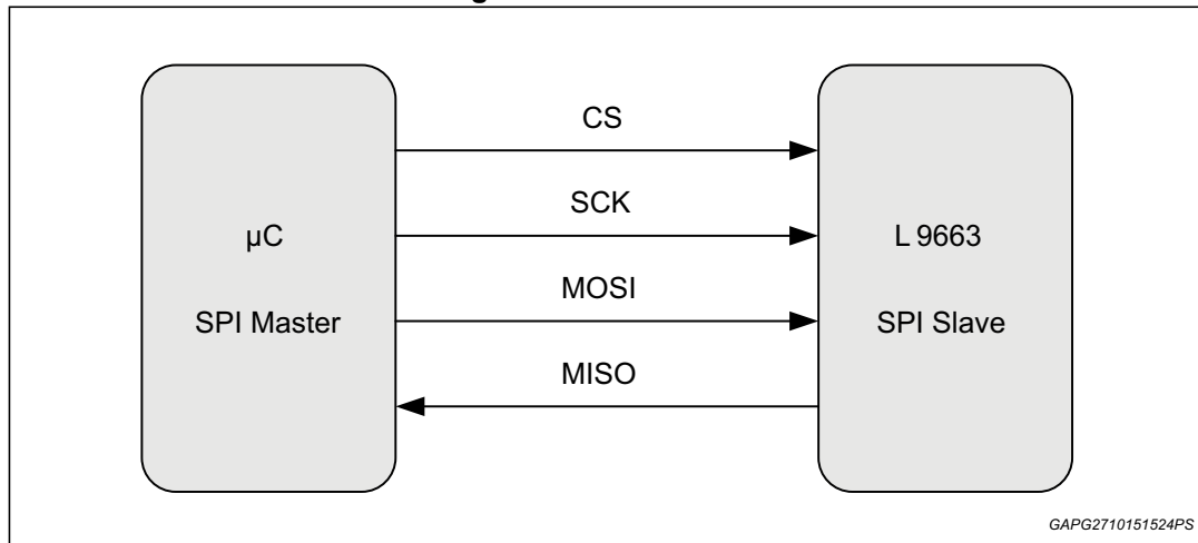
Figure 26. SPI interface
