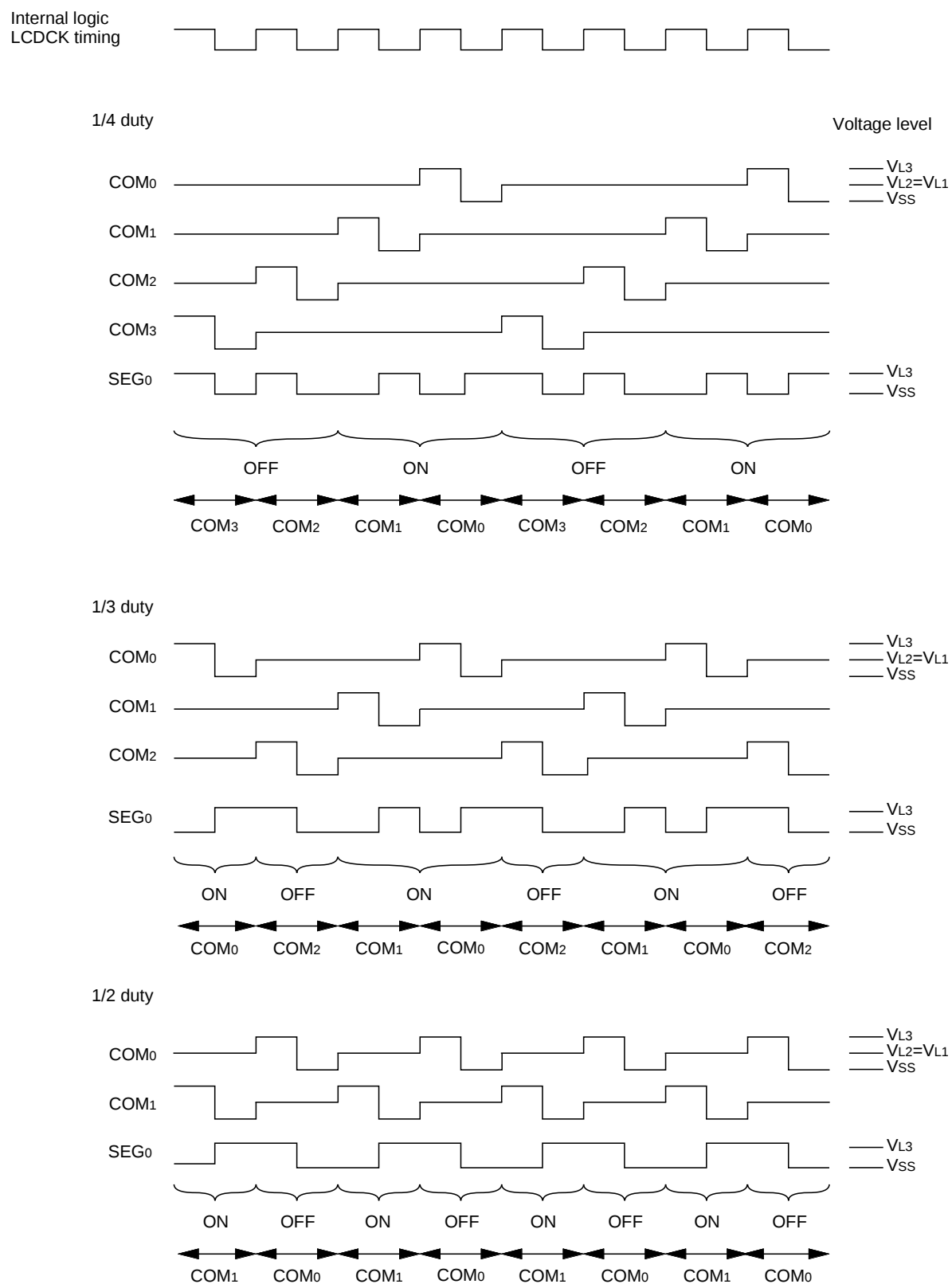
Fig. 40 LCD drive waveform (1/2 bias)
