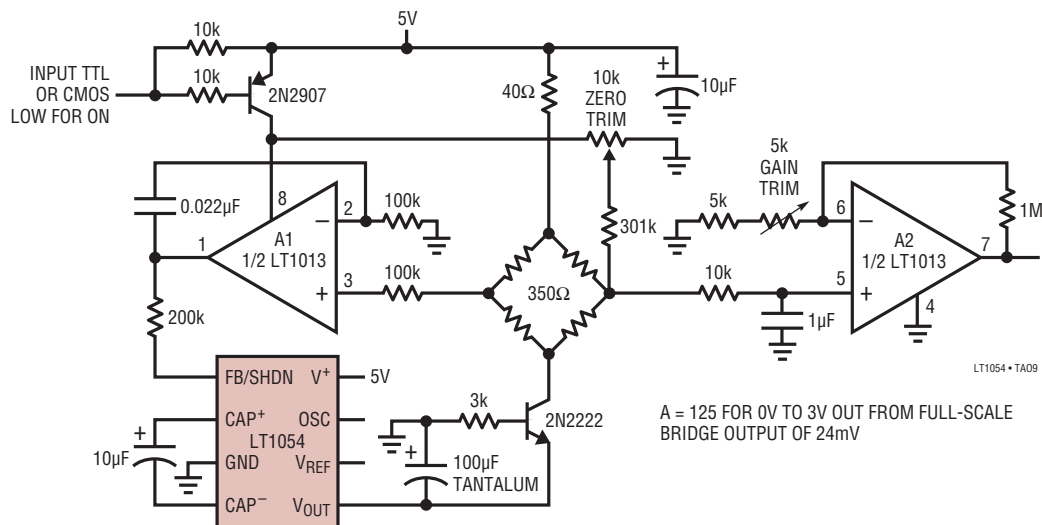
Strain Gauge Bridge Signal Conditioner
