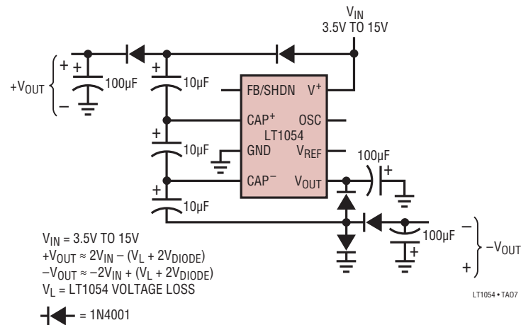
5V to \pm 12V Converter
