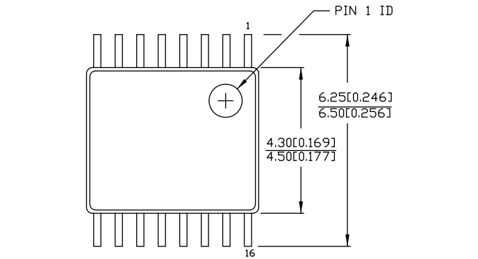
Figure 6. 16-pin TSSOP 4.40 mm Body Z16.173/ZZ16.173 Package Outline, 51-85091
