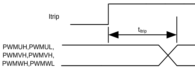
Figure 8 ITRIP timing
