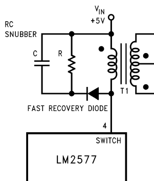
Figure 43. Snubber Circuit
