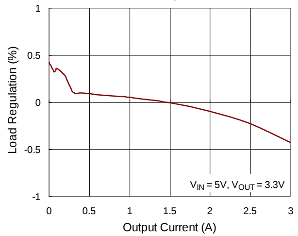
Load Regulation
