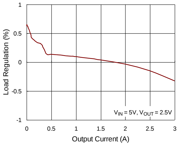
Load Regulation
