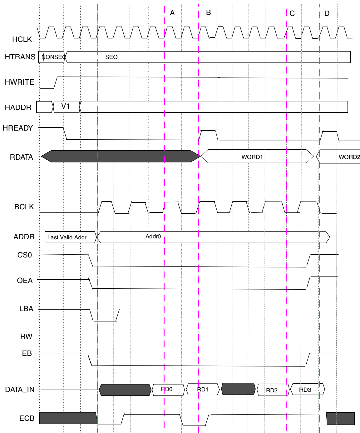
Figure 63. FCE=0,SYNC=1,BCD=1,WSC=4,BCS=0,CSA=0, OEA=0
