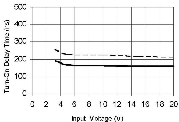
Figure 4C. Turn-On Time vs. Input Voltage
