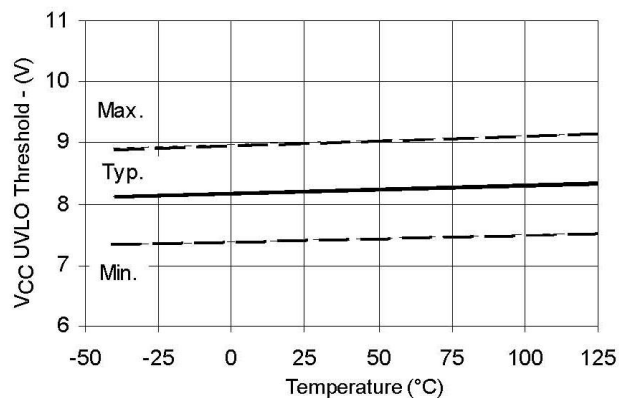
Figure 17B. V CC Undervoltage Threshold(-) vs. Temperature
