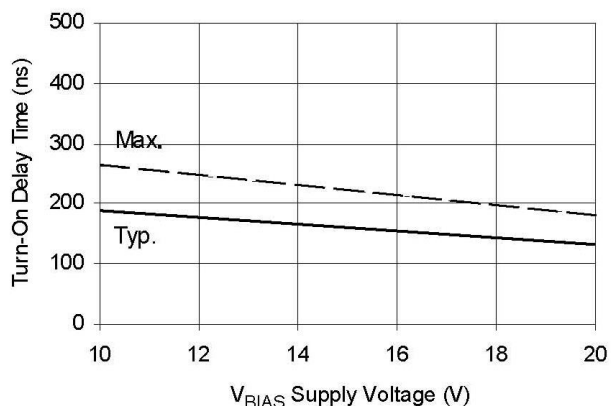
Figure 4B. Turn-On Time vs. Supply Voltage
