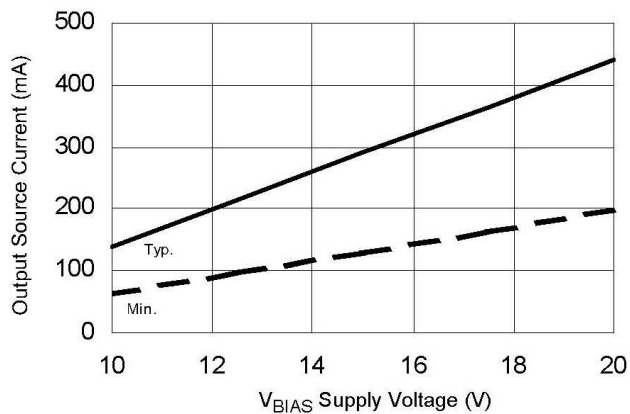
Figure 18B. Output Source Current vs. Supply Current
