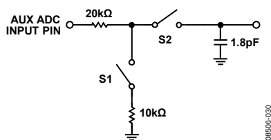
Figure 31. Auxiliary ADC Input Circuit
