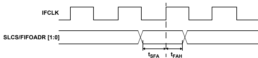
Figure 18. Slave FIFO Synchronous Address Timing Diagram [34]
